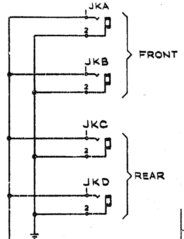
FIG 3 BATTERY JACK (ONE PER RACK)
