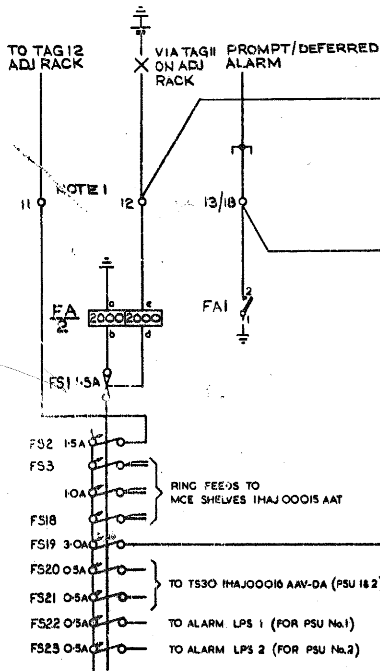
FIG 1 FUSE ALARM (ONE PER RACK)
