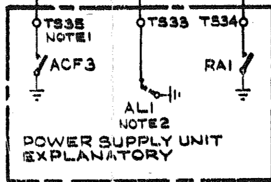
FIG 4 POWER SUPPLY UNIT (TWO PER RACK)
